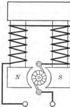
Plan of series wound action.
